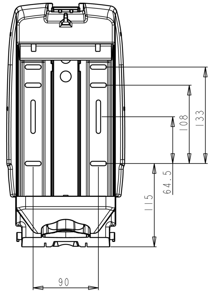
Drill pattern
